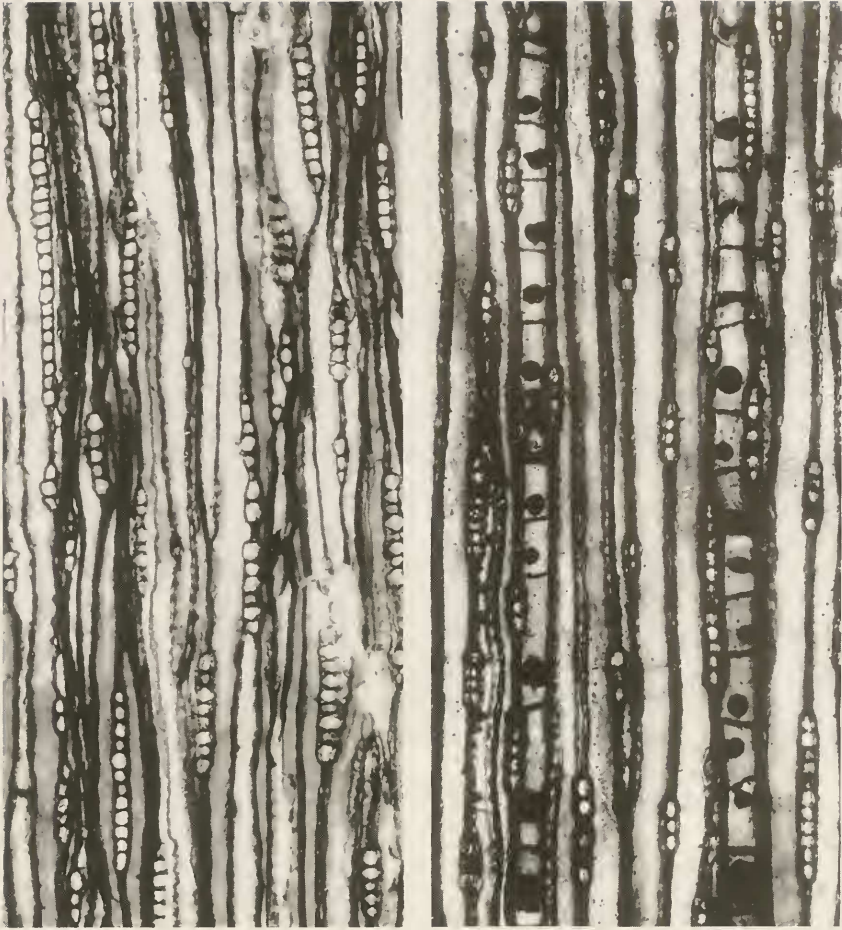
Fig. 3. Taxodioxyton sp., Mine Bilina, No. 4. Longitudinal tangential sections; left ( \times 80 ) uniseriate homocellular rays; right ( \times 90 ) two axial strands of parenchyma cells with dark circular deposits.
